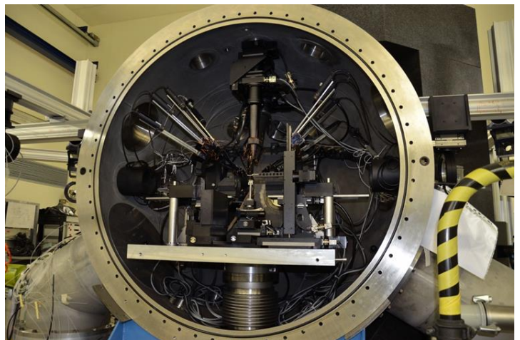
The experimental chamber of the ABC facility with the lid open. Multiple diagnostics are mounted and functioning in every shot.
